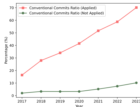
Fig. 5: Application Trend of Conventional Commits Specification in Developers' Commits
